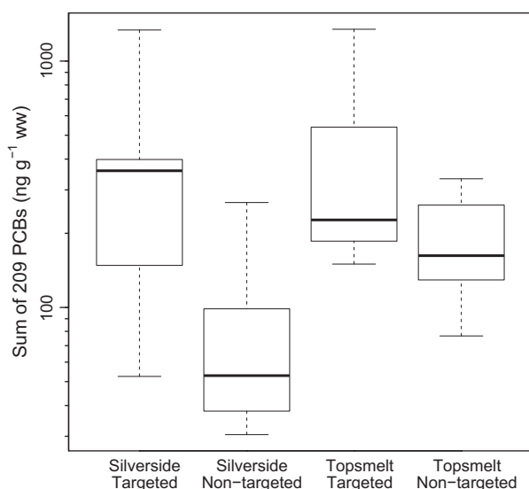
Fig. 2. Box and whisker plot of PCB wet weight concentrations across species and site type (targeted versus non-targeted). Thick line represents median concentration, box represents 25th and 75th percentile, and whiskers represent 95% confidence intervals. Note: log scale.
